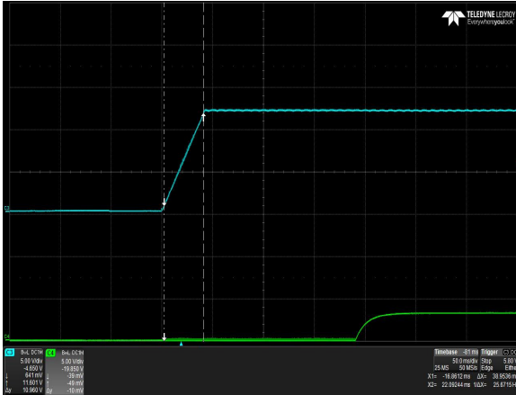
Figure 7: DS1600SPE-3 Output Voltage Startup Characteristic Vin = 90Vac Load: I_O = 63.2A I_{SB} = 3.5A Ch 3: V_O Ch 4: Pwr_GOOD
