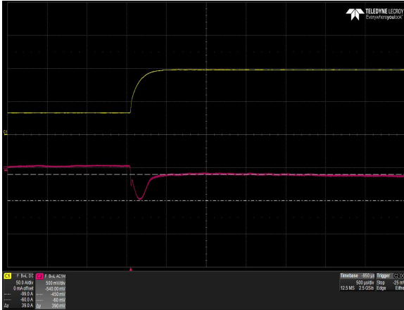
Figure 13: DS1600SPE-3 Transient Response - V_O Deviation 25% to 75% load change 1A/uS slew rate V_{in} = 230V_{ac} Ch 1: I_o Ch 2: V_O Output capacitance=2350uF
