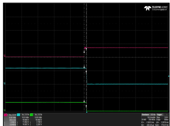
Figure 12: DS1600SPE-3 Turn Off Characteristic via PS_KILL_L Load: I_O = 129.8A I_{SB} = 3.5A Ch 2: PS_KILL_L Ch 3: V_O Ch 4: Pwr_GOOD
