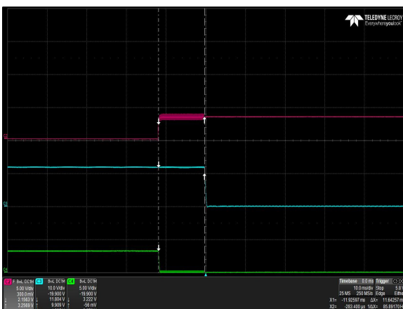
Figure 11: DS1600SPE-3 Turn Off Characteristic via PS_ON_L Load: I_O = 129.8A I_{SB} = 3.5A Ch 2: PS_ON_L Ch 3: V_O Ch 4: Pwr_GOOD
