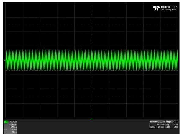
Figure 10: DS1600SPE-3 Ripple and Noise Measurement Vin = 180Vac Load: I_O = 129.8A I_{SB} = 3.5A Ch 4: V_O
