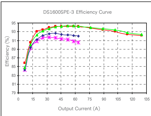
Figure 15: DS1600SPE-3 Efficiency Curve @ 25°C Loading: I_{o\_main} = 10\%I_{o\_max} increment to 129.8A, I_{SB} = 3.5A
