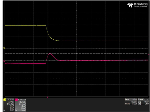
Figure 14: DS1600SPE-3 Transient Response - V_O Deviation 75% to 25% load change 1A/uS slew rate V_{in} = 230V_{ac} Ch 1: I_o Ch 2: V_O Output capacitance=2350uF
