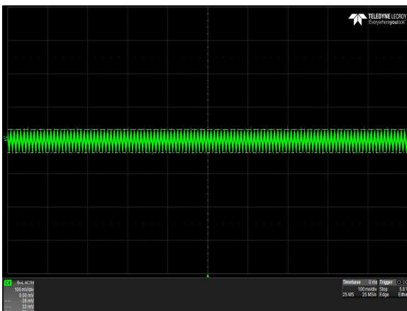
Figure 9: DS1600SPE-3 Ripple and Noise Measurement Vin = 90Vac Load: I_O = 63.2A I_{SB} = 3.5A Ch 4: V_O
